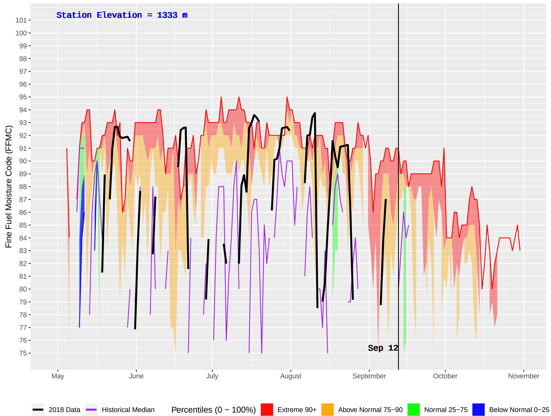
GOLDSTREAM 2 (919) : Historical (2005–2016) and Current (2018) Daily Fine Fuel Moisture Code (FFMC)
